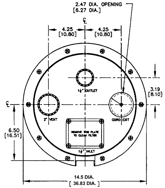
TOP VIEW OF COVER
