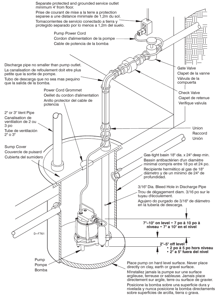
Figure 1. Typical Installation • Installation Type • Instalacion Tipica
